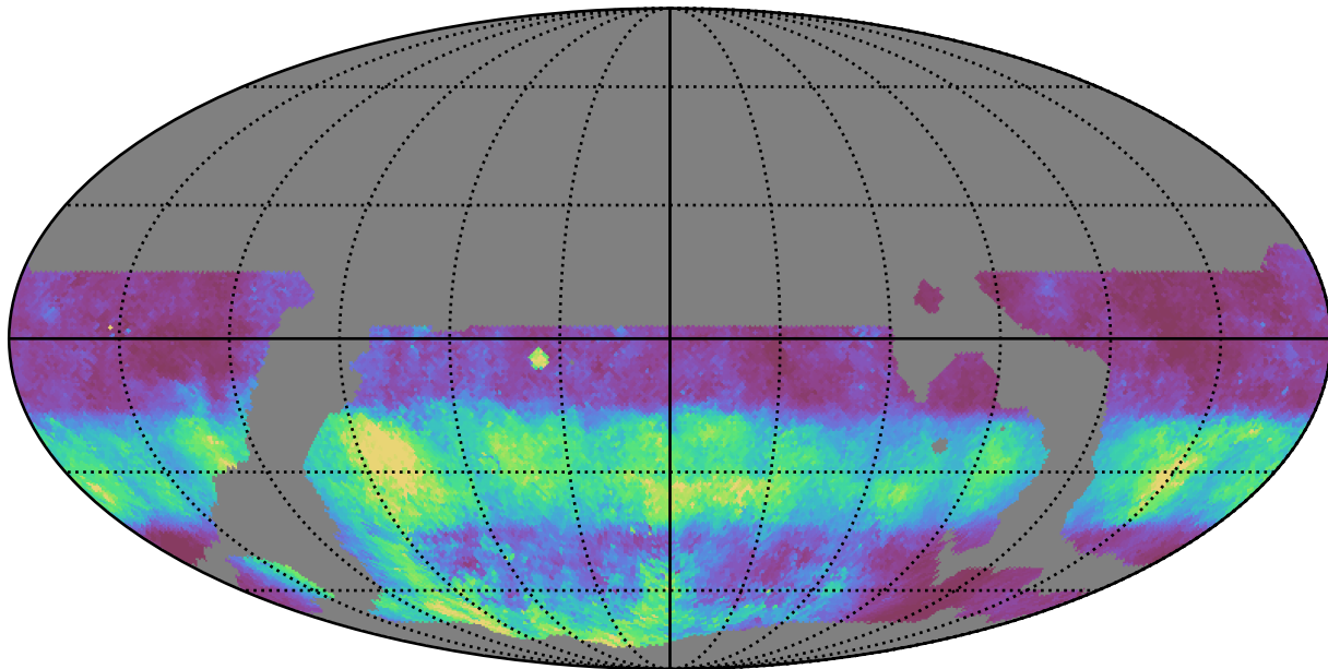
weather_cloudso18v3.4_10yrs WFD g band: Median normairmass
