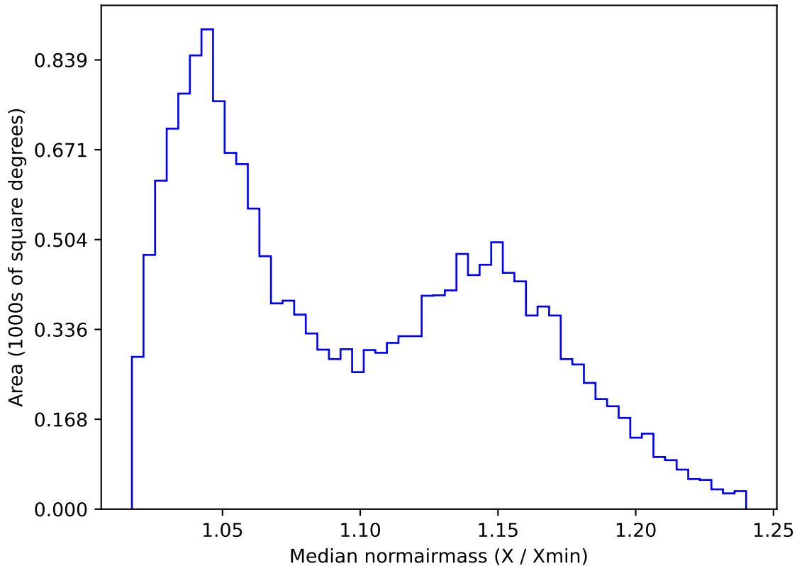
weather_cloudso18v3.4_10yrs WFD g band: Median normairmass
