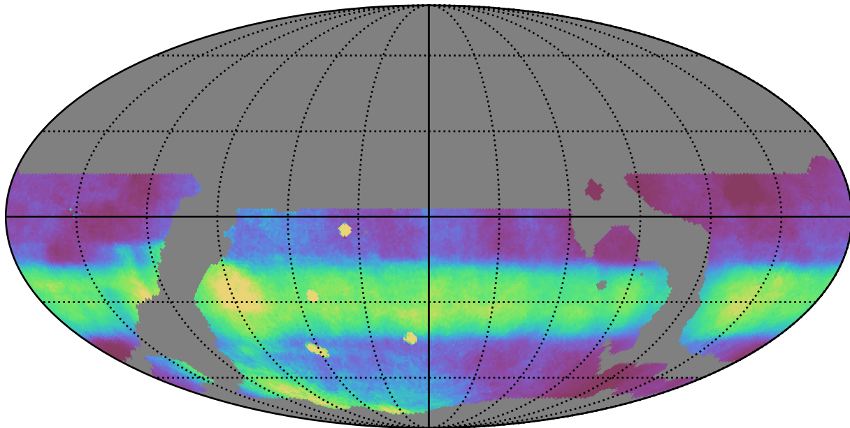
weather_cloudso18v3.4_10yrs WFD all bands: Median normairmass
