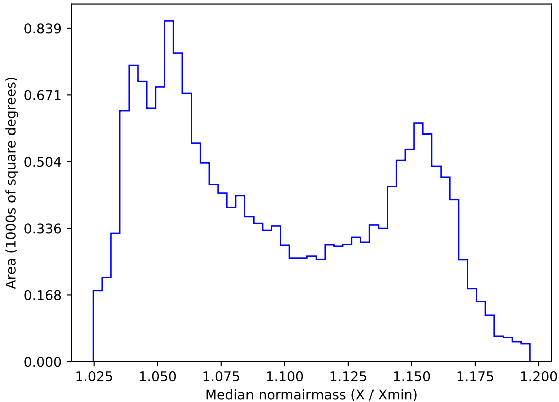
weather_cloudso18v3.4_10yrs WFD all bands: Median normairmass
