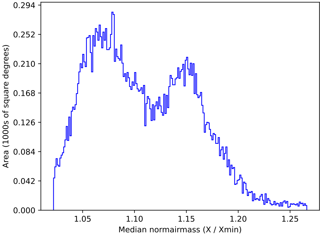
weather_cloudso18v3.4_10yrs All sky y band: Median normairmass
