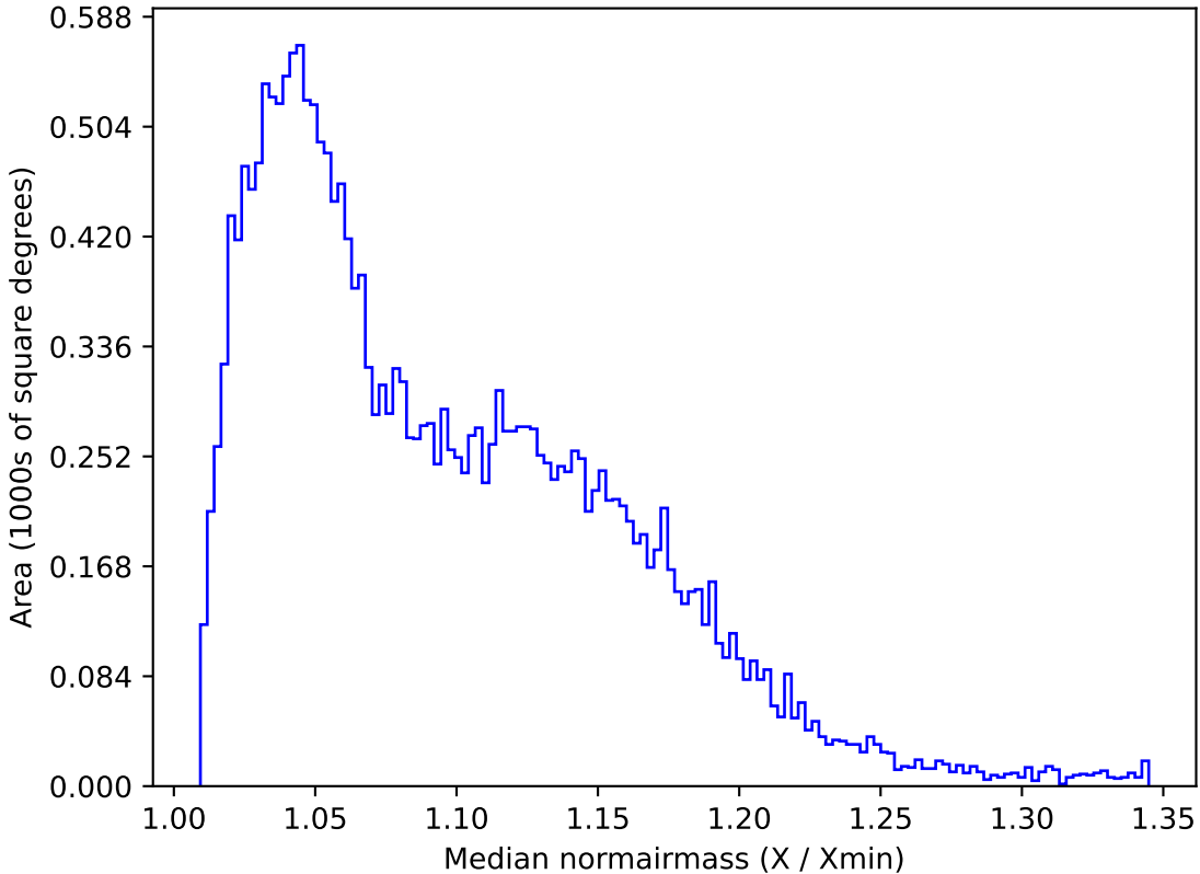
weather_cloudso18v3.4_10yrs All sky u band: Median normairmass
