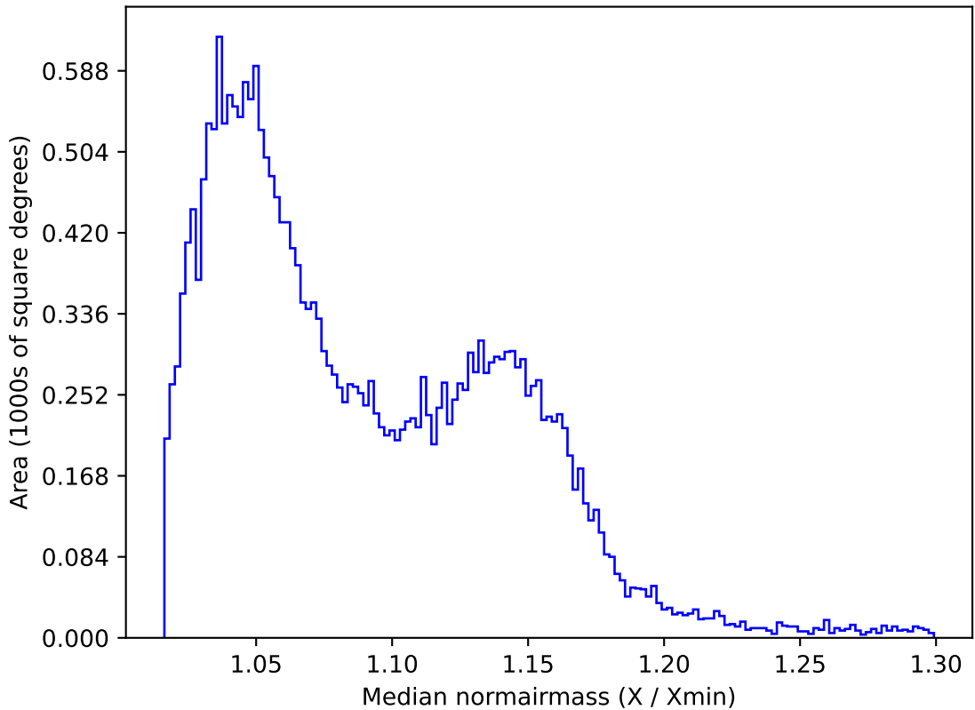
weather_cloudso18v3.4_10yrs All sky r band: Median normairmass
