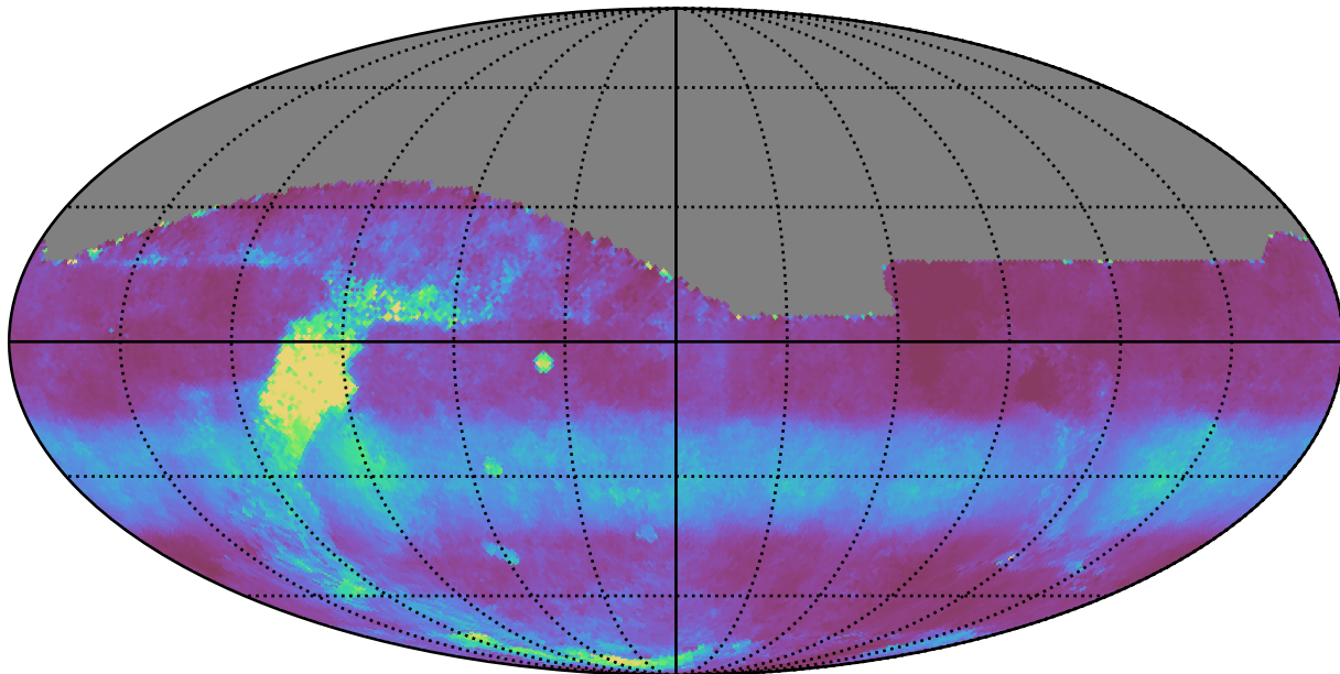
weather_cloudso18v3.4_10yrs All sky i band: Median normairmass
