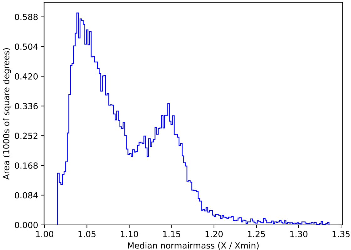
weather_cloudso18v3.4_10yrs All sky i band: Median normairmass
