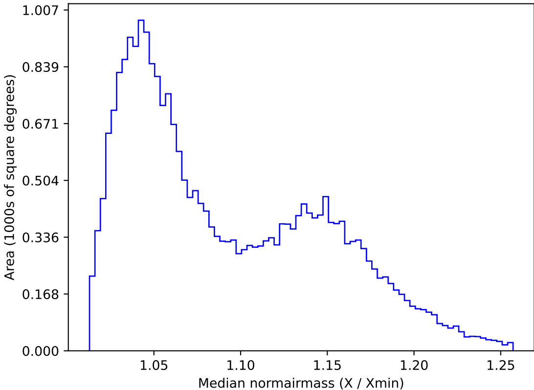
weather_cloudso18v3.4_10yrs All sky g band: Median normairmass
