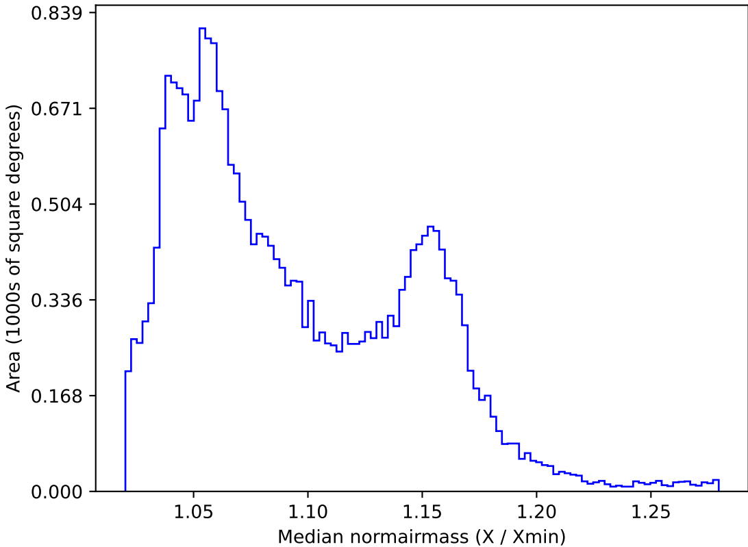
weather_cloudso18v3.4_10yrs All sky all bands: Median normairmass
