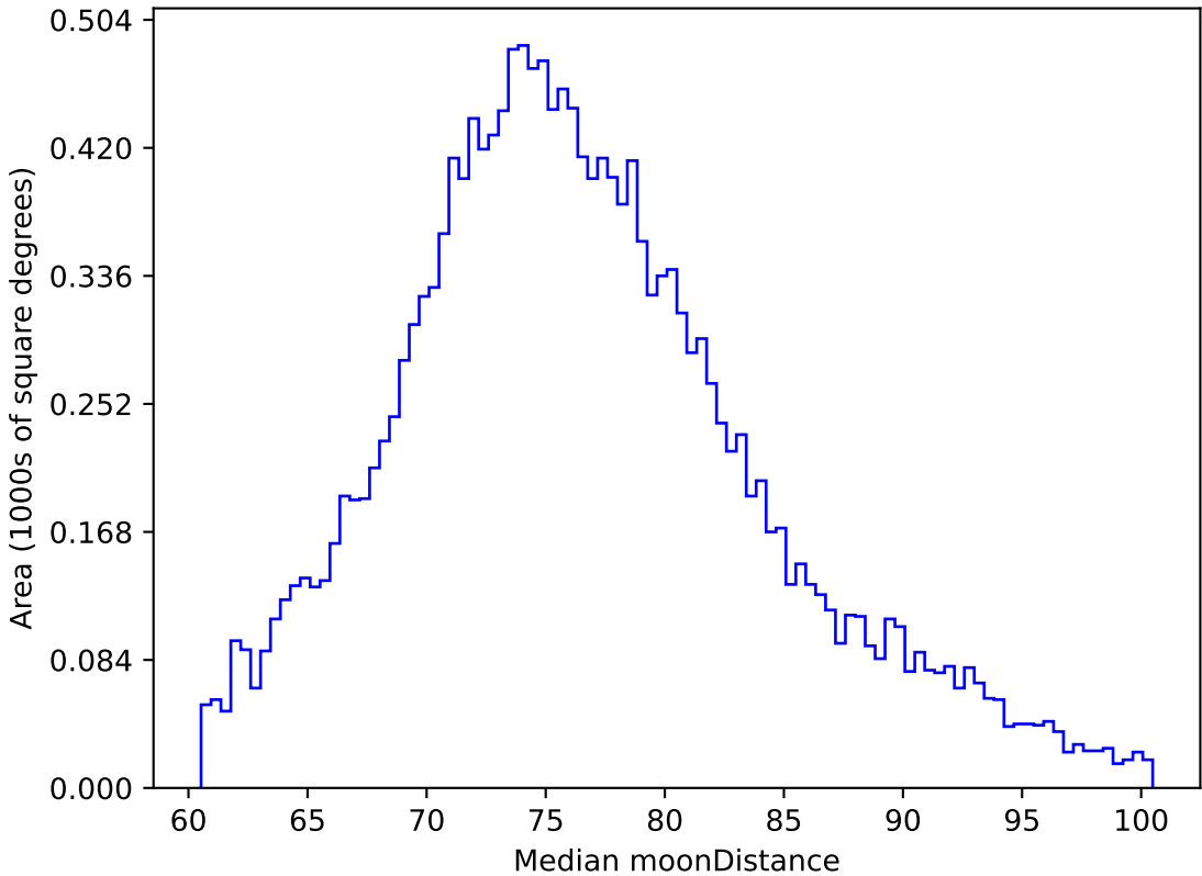
weather_cloudso18v3.4_10yrs WFD z band: Median moonDistance
