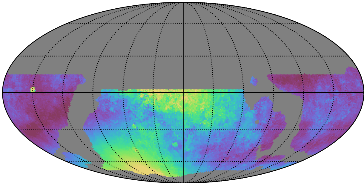
weather_cloudso18v3.4_10yrs WFD y band: Median moonDistance
