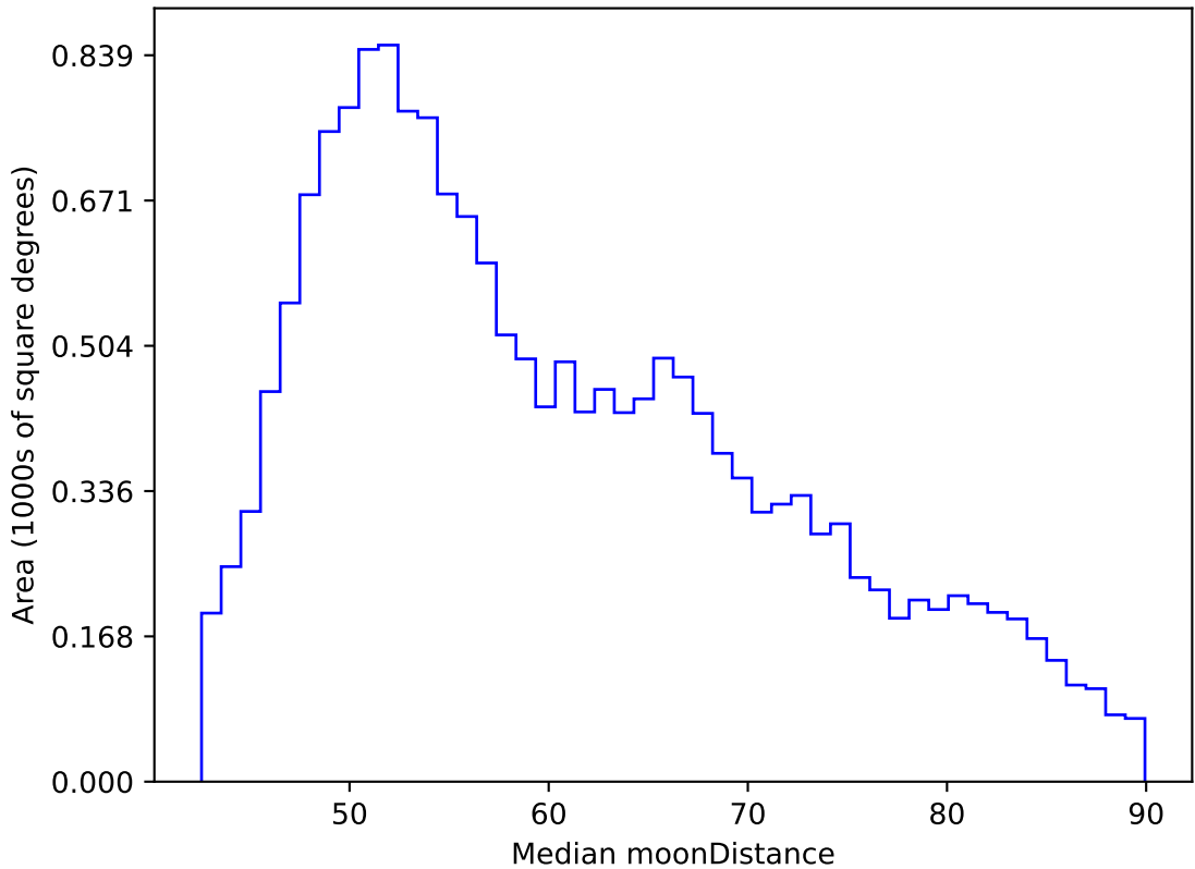
weather_cloudso18v3.4_10yrs WFD y band: Median moonDistance
