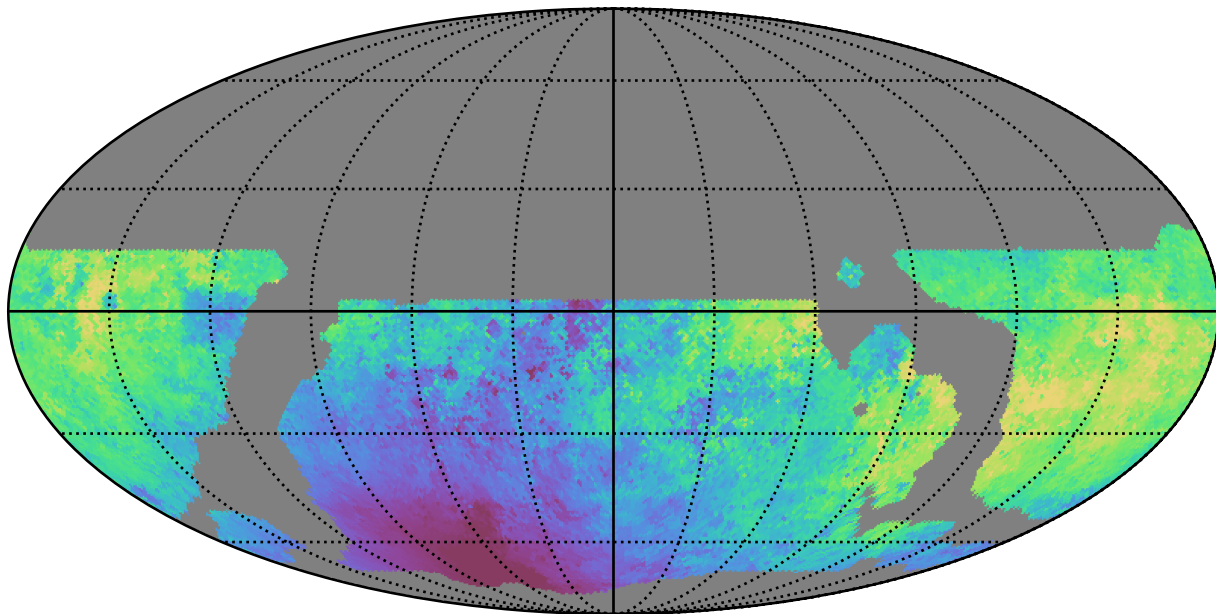
weather_cloudso18v3.4_10yrs WFD u band: Median moonDistance
