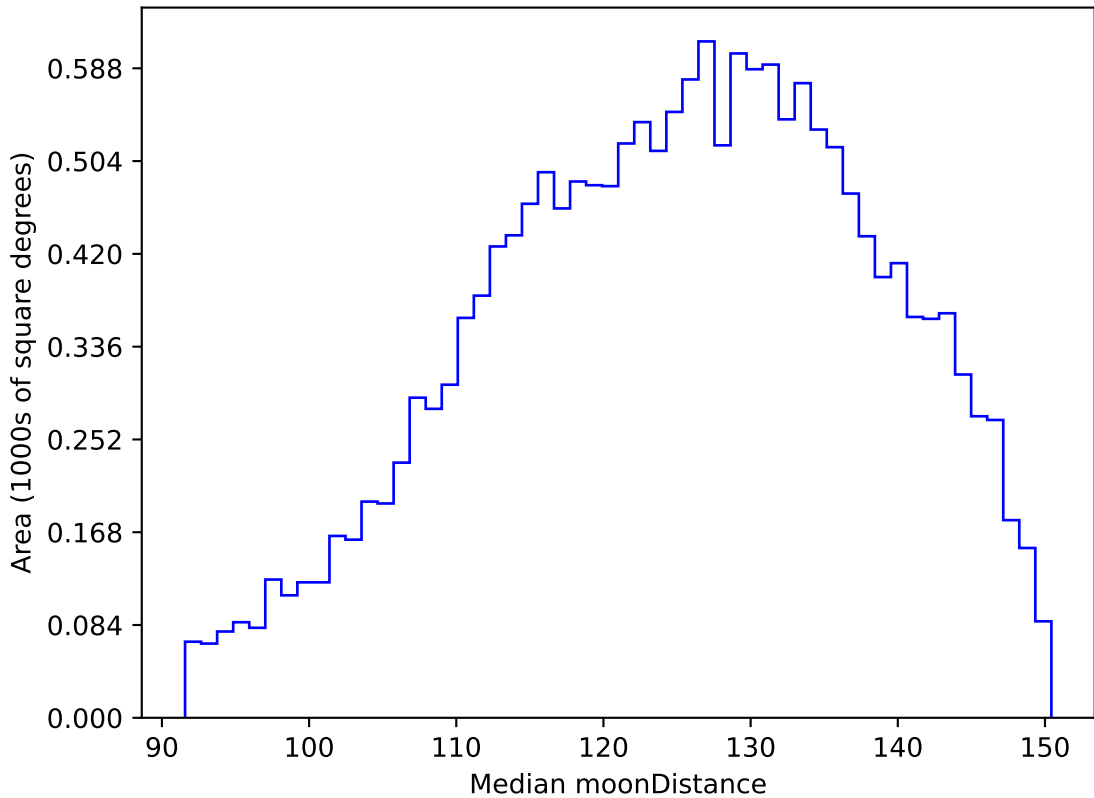
weather_cloudso18v3.4_10yrs WFD u band: Median moonDistance
