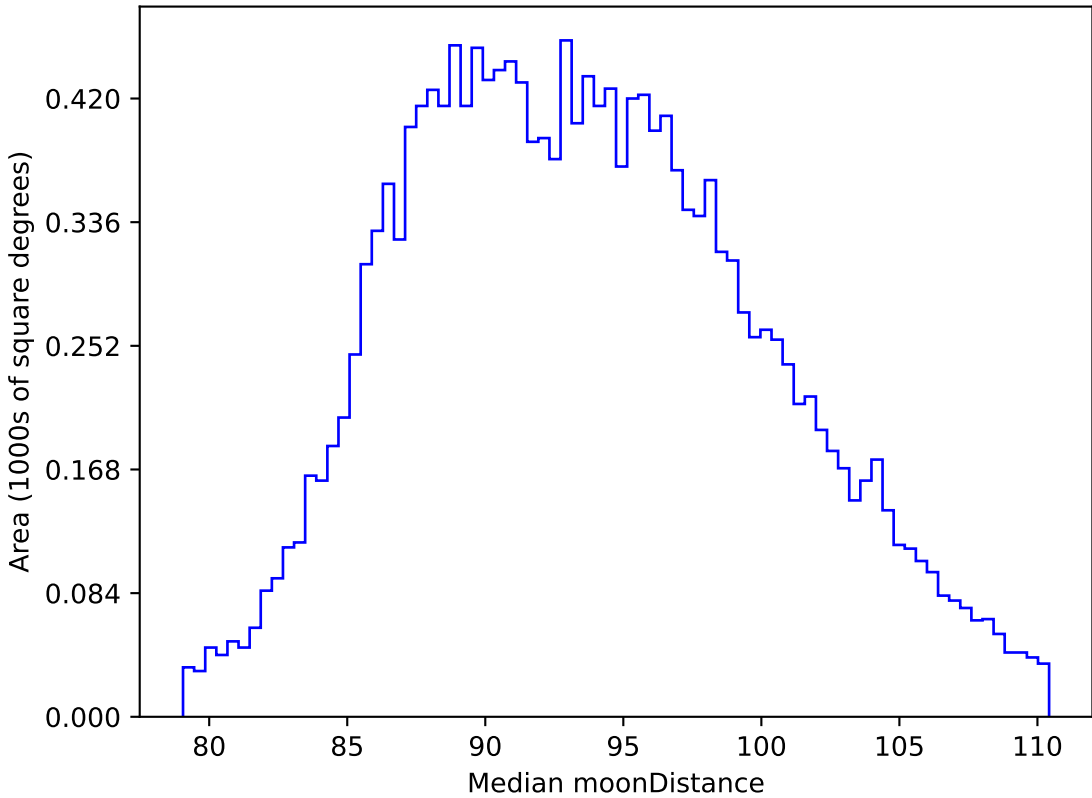
weather_cloudso18v3.4_10yrs WFD i band: Median moonDistance
