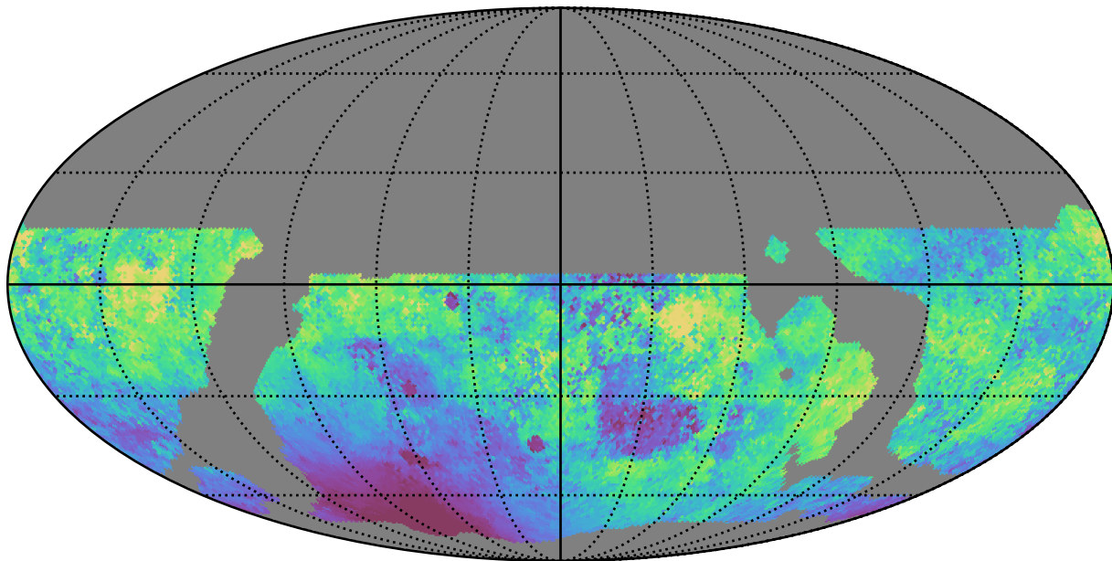
weather_cloudso18v3.4_10yrs WFD g band: Median moonDistance
