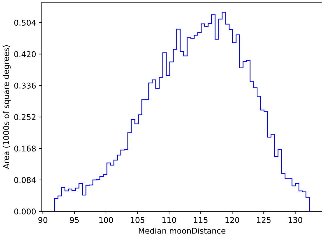
weather_cloudso18v3.4_10yrs WFD g band: Median moonDistance
