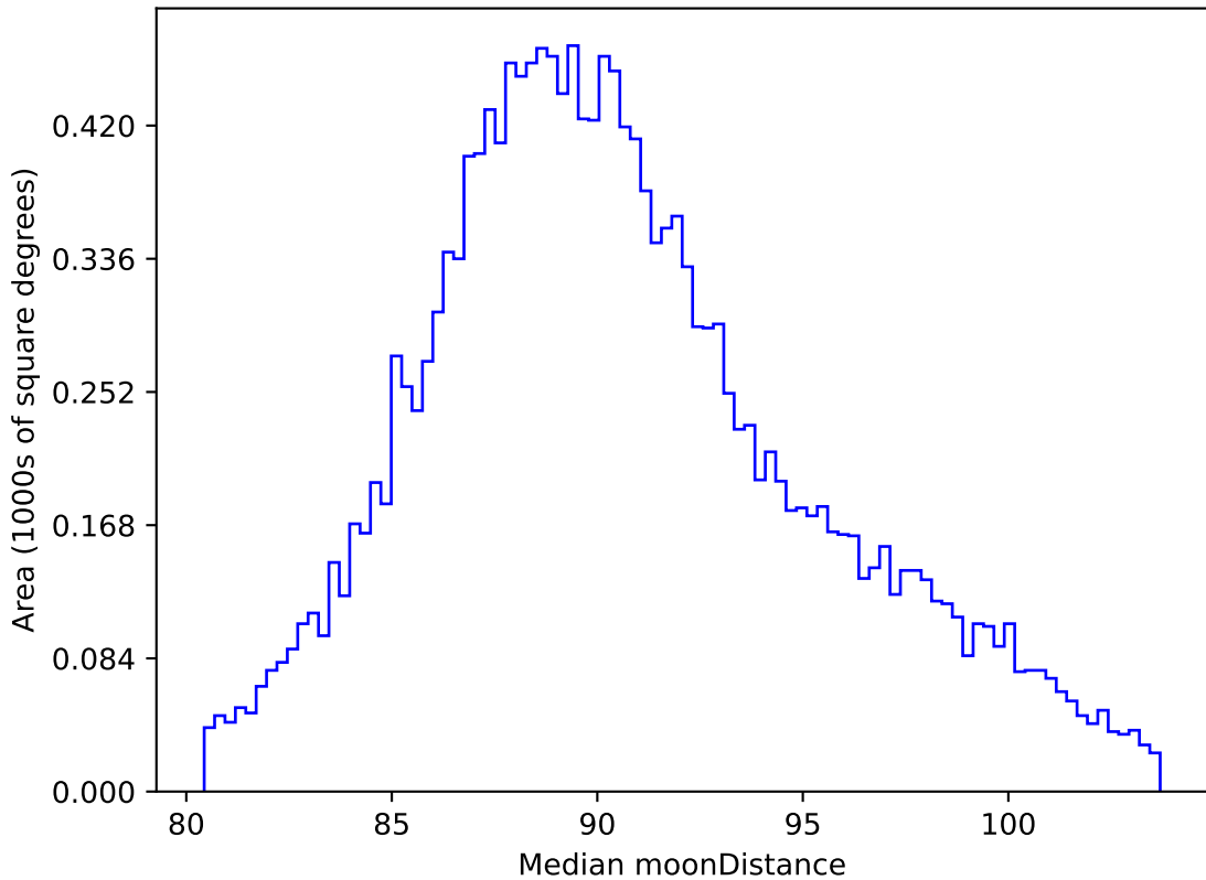
weather_cloudso18v3.4_10yrs WFD all bands: Median moonDistance
