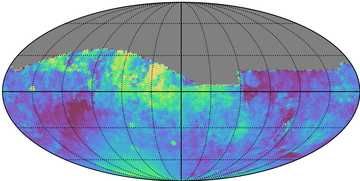
weather_cloudso18v3.4_10yrs All sky z band: Median moonDistance
