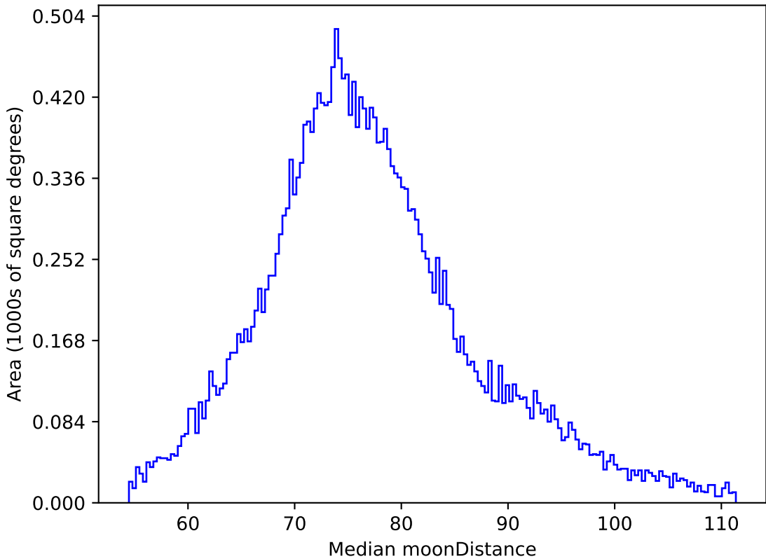
weather_cloudso18v3.4_10yrs All sky z band: Median moonDistance
