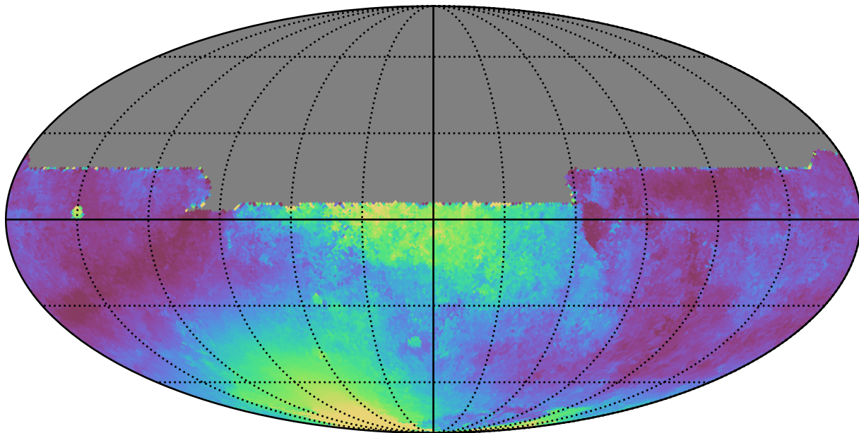
weather_cloudso18v3.4_10yrs All sky y band: Median moonDistance
