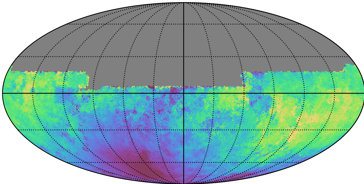
weather_cloudso18v3.4_10yrs All sky u band: Median moonDistance
