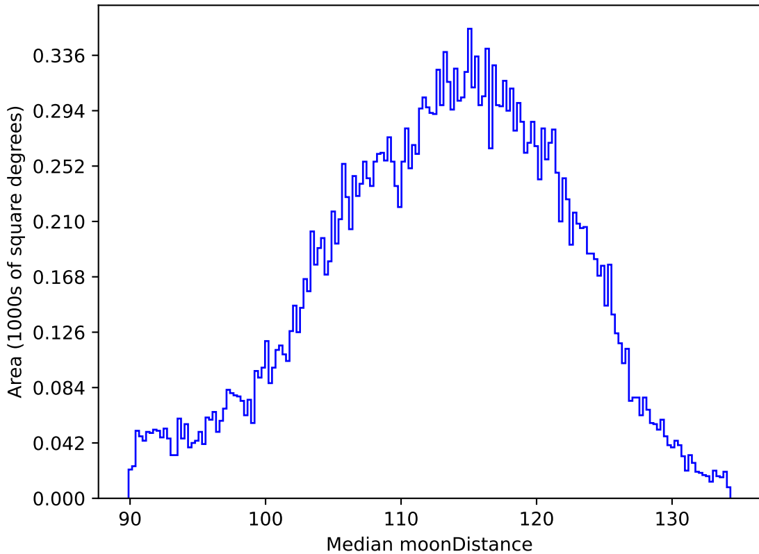
weather_cloudso18v3.4_10yrs All sky r band: Median moonDistance
