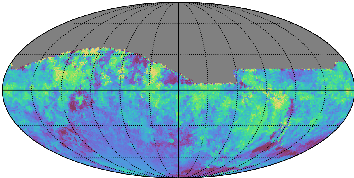
weather_cloudso18v3.4_10yrs All sky i band: Median moonDistance
