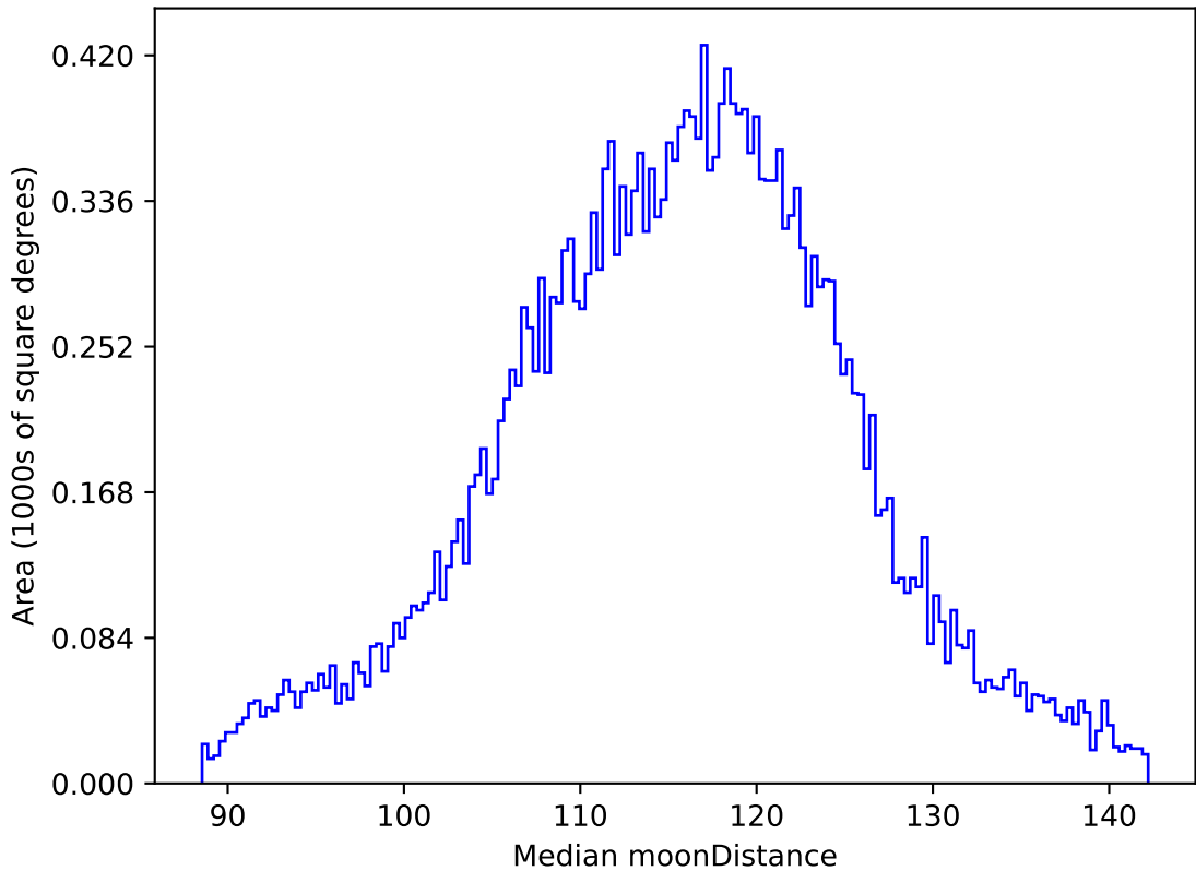
weather_cloudso18v3.4_10yrs All sky g band: Median moonDistance
