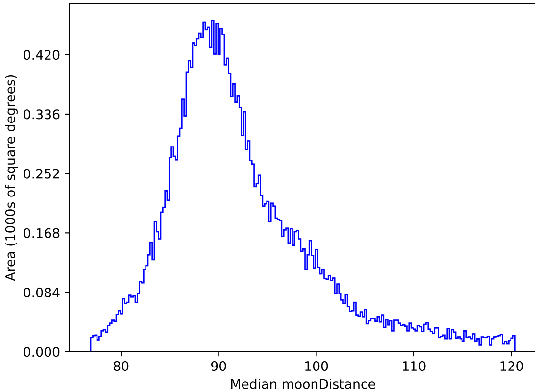
weather_cloudso18v3.4_10yrs All sky all bands: Median moonDistance
