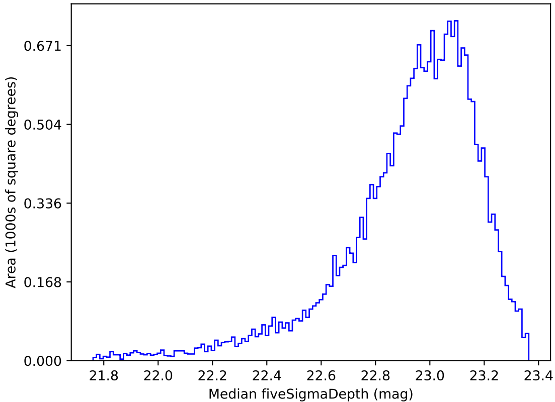
weather_cloudso18v3.4_10yrs Yr 1 z band: Median fiveSigmaDepth
