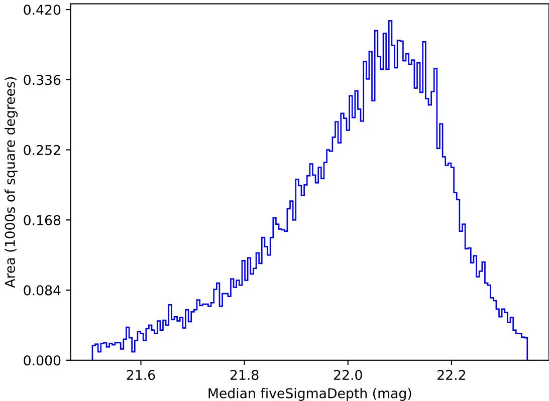
weather_cloudso18v3.4_10yrs Yr 1 y band: Median fiveSigmaDepth
