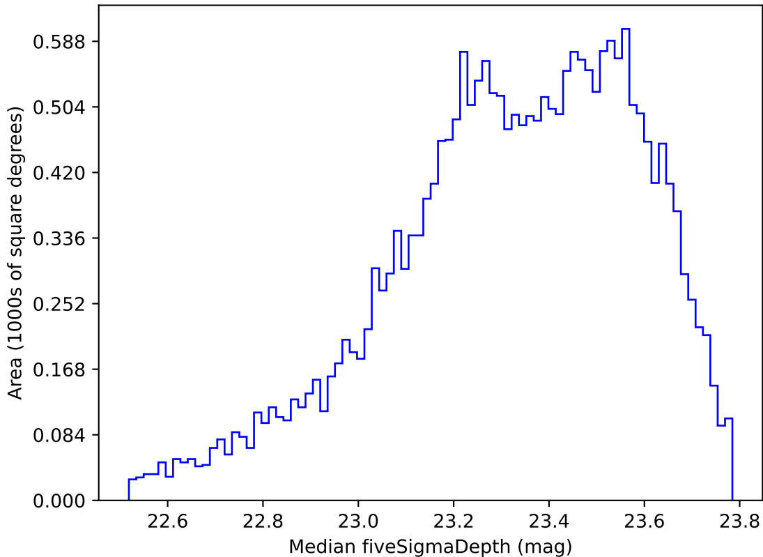
weather_cloudso18v3.4_10yrs Yr 1 u band: Median fiveSigmaDepth
