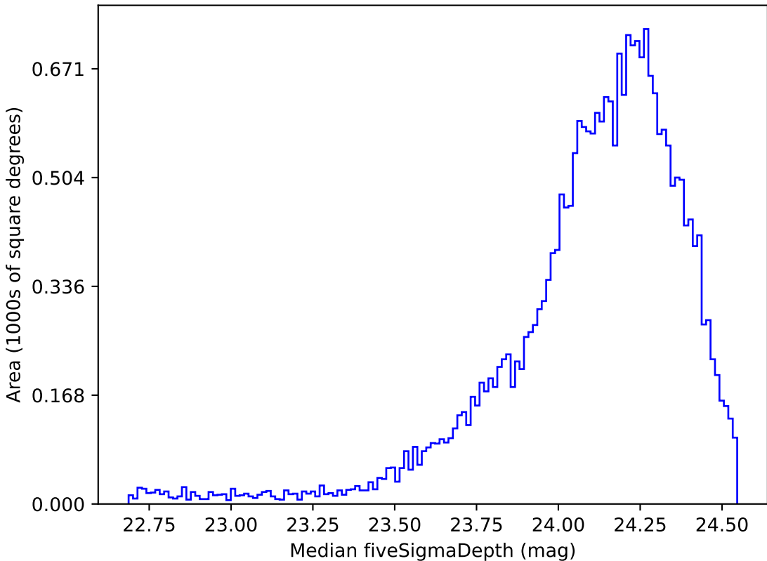
weather_cloudso18v3.4_10yrs Yr 1 r band: Median fiveSigmaDepth
