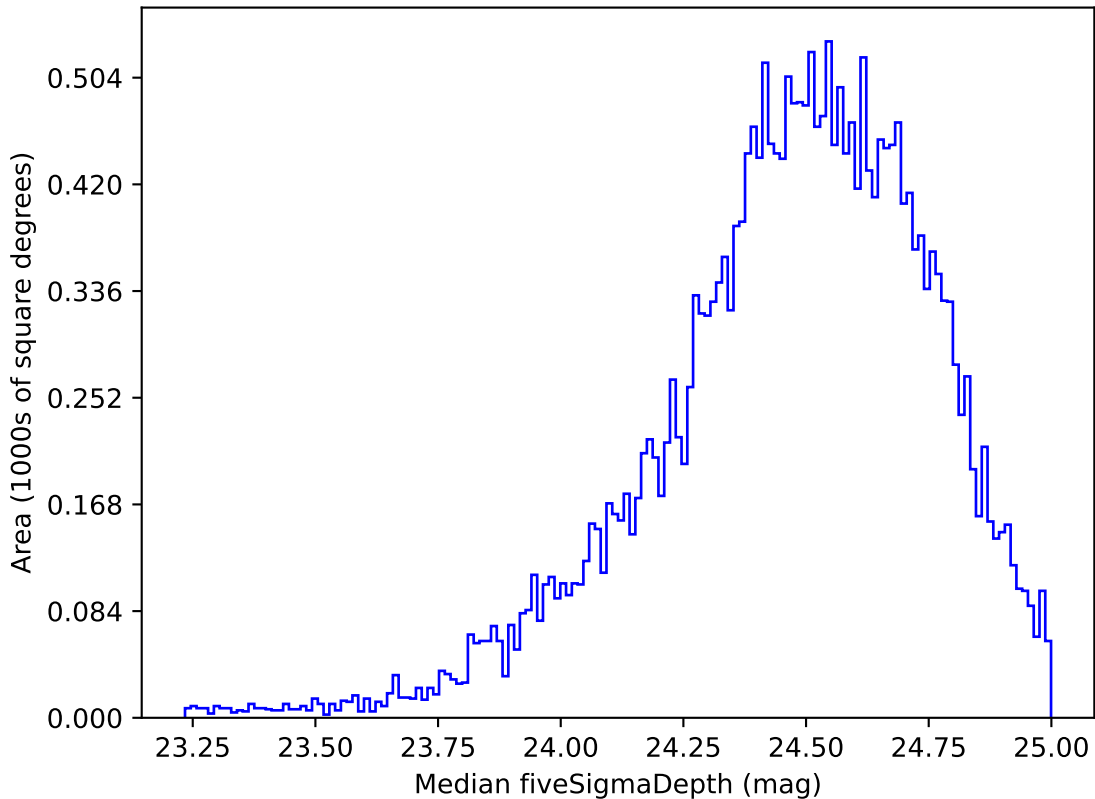
weather_cloudso18v3.4_10yrs Yr 1 g band: Median fiveSigmaDepth
