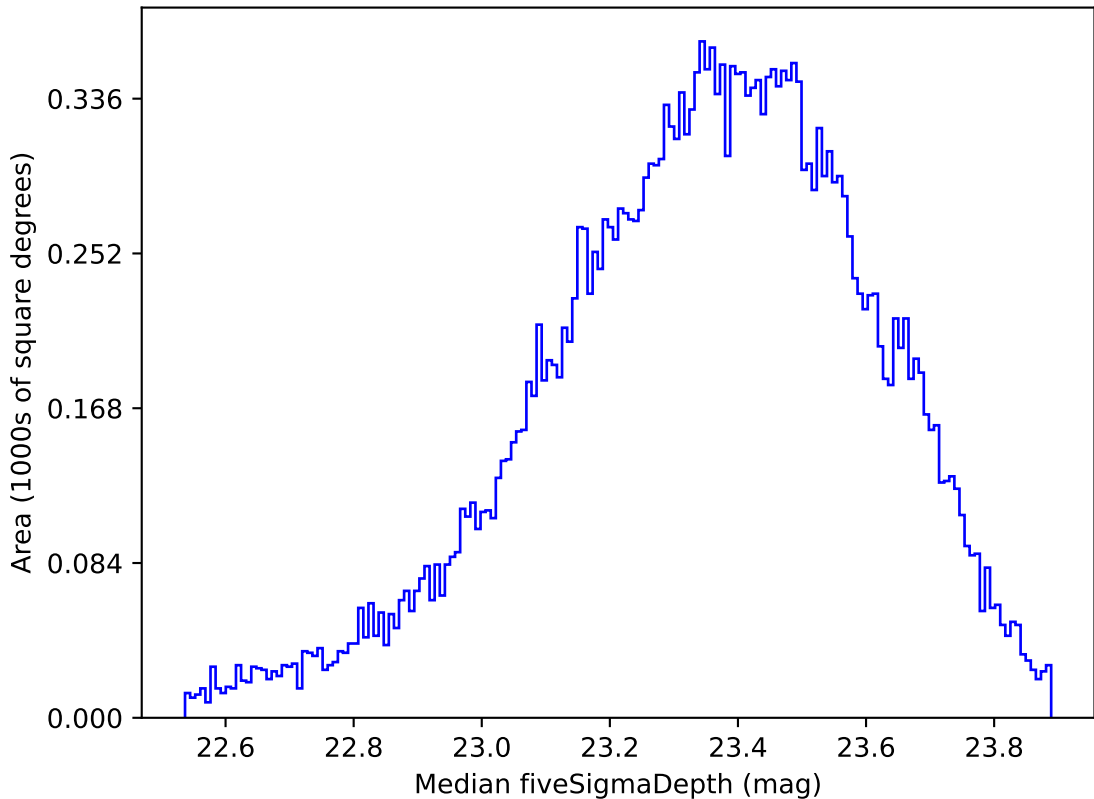
weather_cloudso18v3.4_10yrs Yr 1 all bands: Median fiveSigmaDepth
