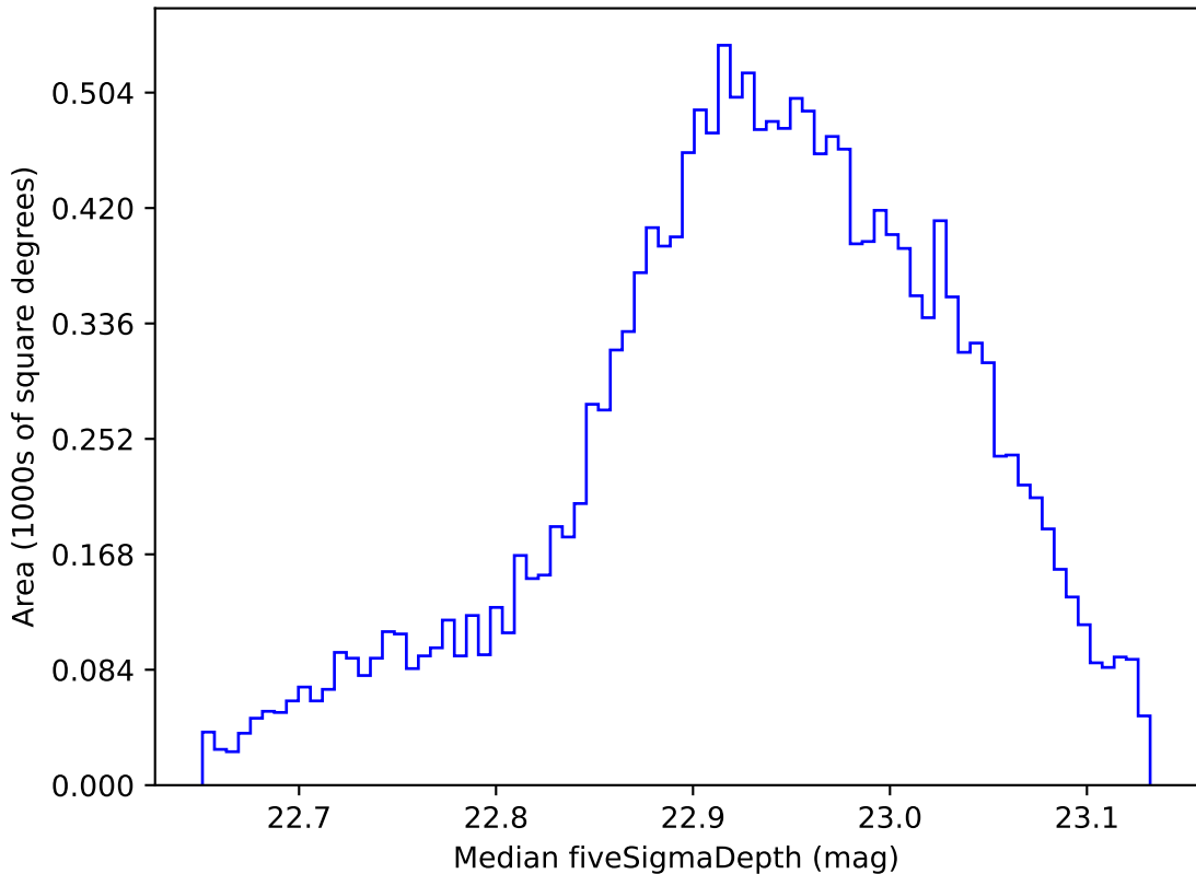
weather_cloudso18v3.4_10yrs WFD z band: Median fiveSigmaDepth
