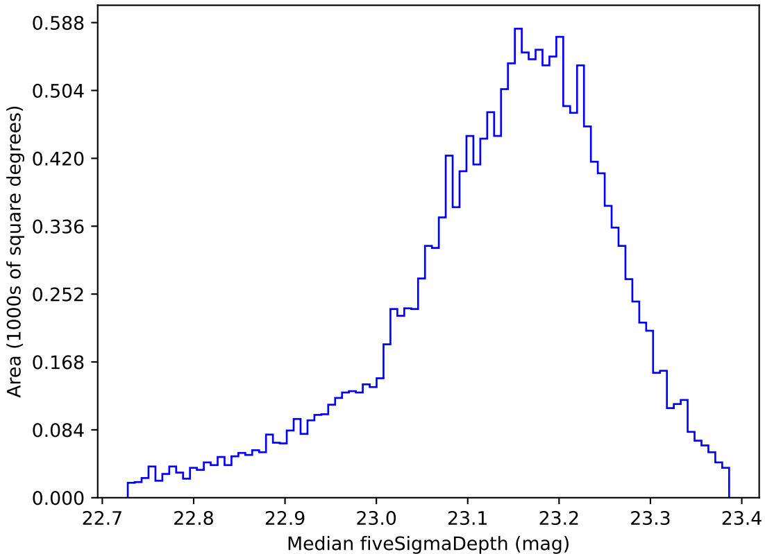
weather_cloudso18v3.4_10yrs WFD u band: Median fiveSigmaDepth
