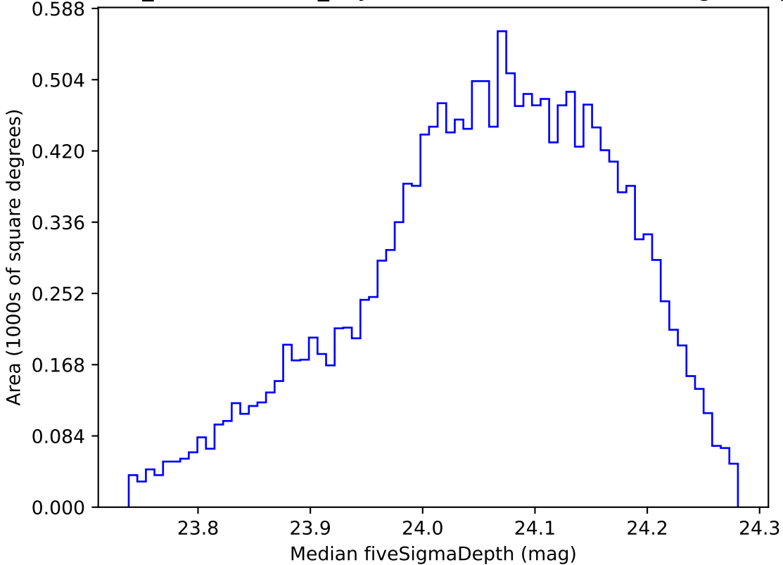
weather_cloudso18v3.4_10yrs WFD r band: Median fiveSigmaDepth
