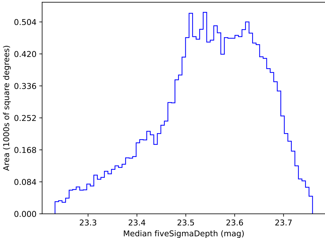
weather_cloudso18v3.4_10yrs WFD i band: Median fiveSigmaDepth
