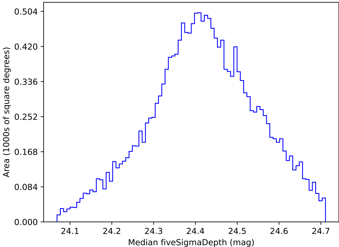
weather_cloudso18v3.4_10yrs WFD g band: Median fiveSigmaDepth
