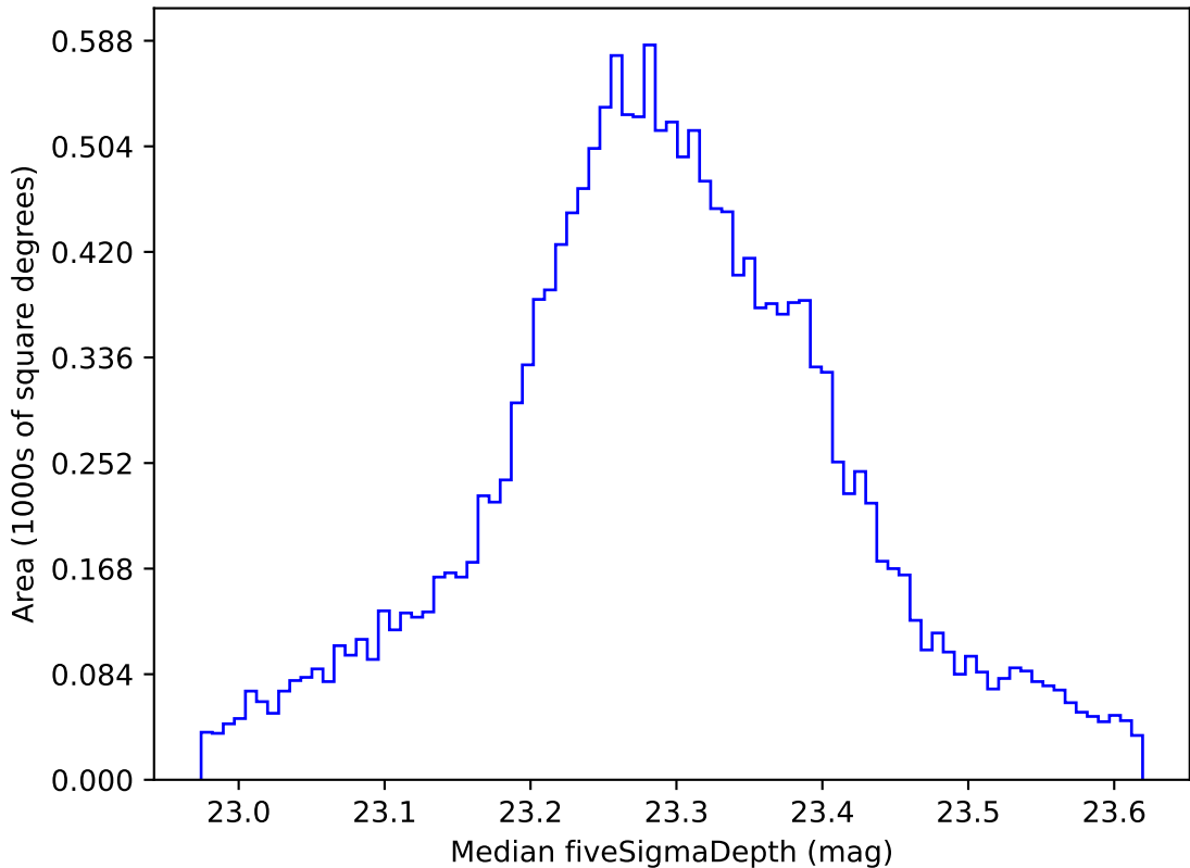
weather_cloudso18v3.4_10yrs WFD all bands: Median fiveSigmaDepth
