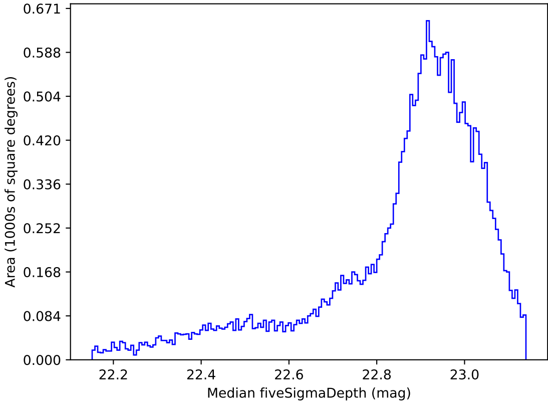
weather_cloudso18v3.4_10yrs All sky z band: Median fiveSigmaDepth
