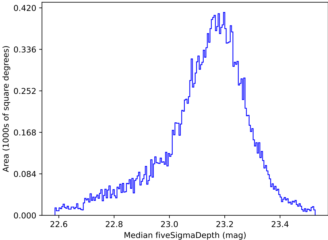
weather_cloudso18v3.4_10yrs All sky u band: Median fiveSigmaDepth
