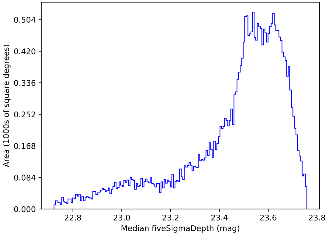
weather_cloudso18v3.4_10yrs All sky i band: Median fiveSigmaDepth
