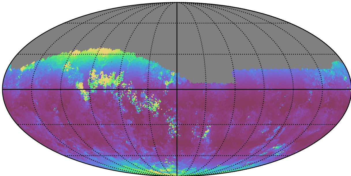
weather_cloudso18v3.4_10yrs Yr 1 z band: Median airmass
