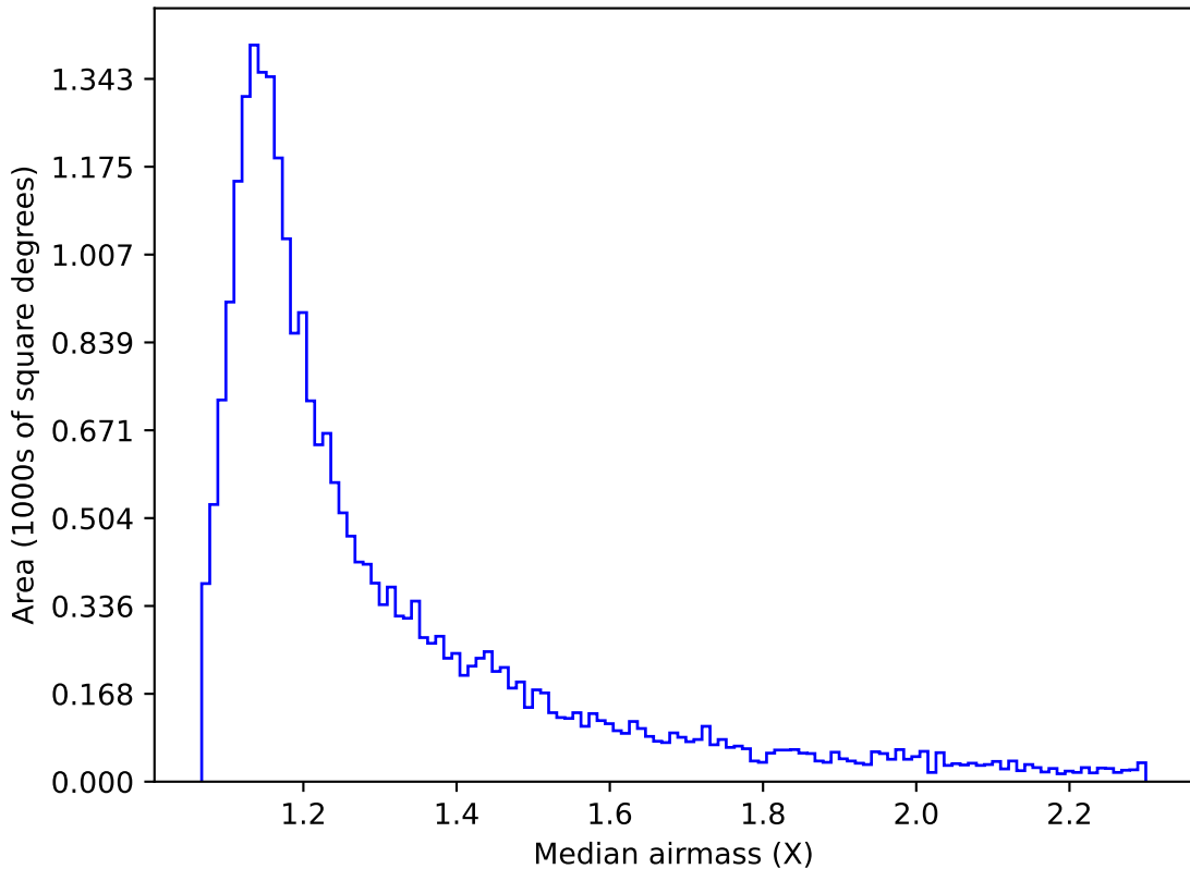
weather_cloudso18v3.4_10yrs Yr 1 z band: Median airmass
