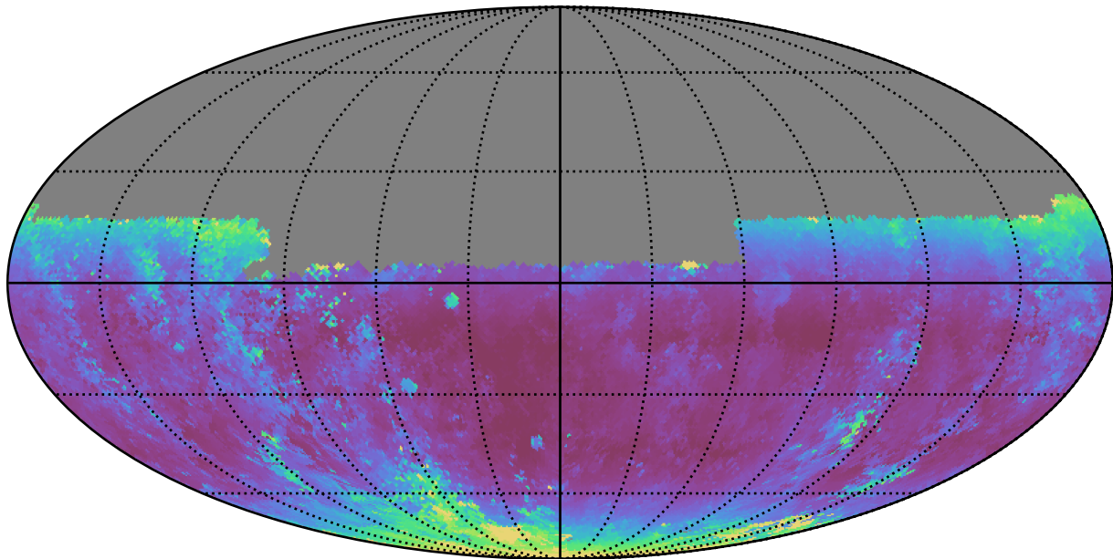
weather_cloudso18v3.4_10yrs Yr 1 y band: Median airmass
