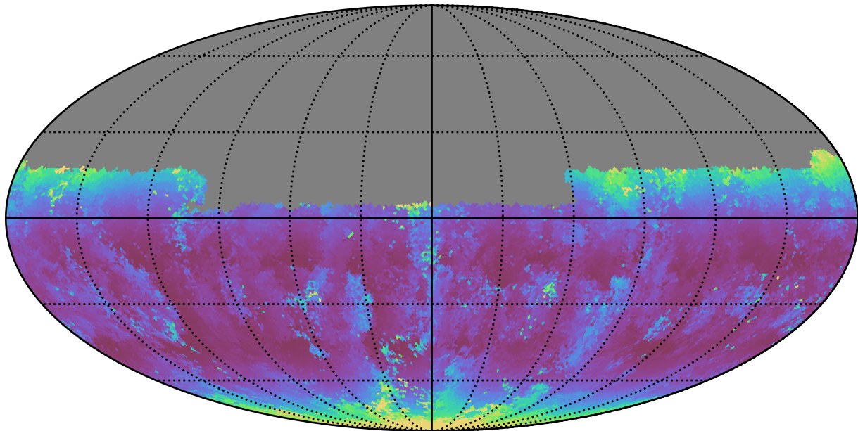
weather_cloudso18v3.4_10yrs Yr 1 u band: Median airmass
