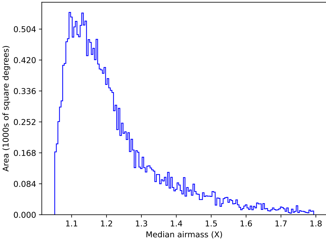
weather_cloudso18v3.4_10yrs Yr 1 u band: Median airmass
