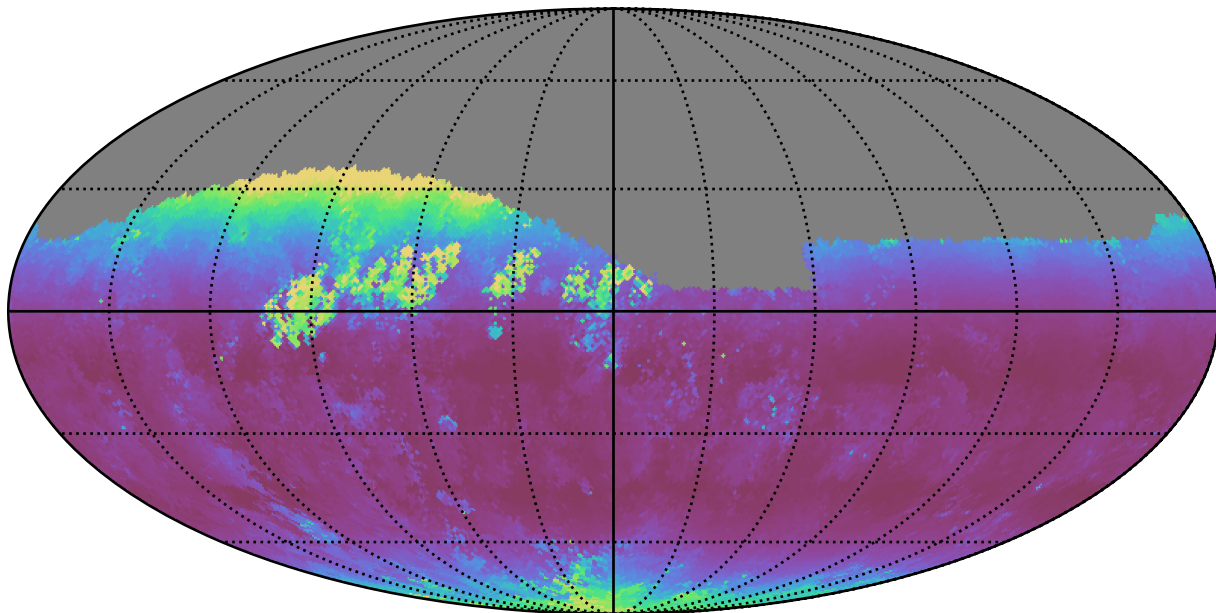
weather_cloudso18v3.4_10yrs Yr 1 r band: Median airmass
