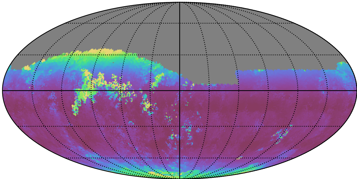
weather_cloudso18v3.4_10yrs Yr 1 i band: Median airmass
